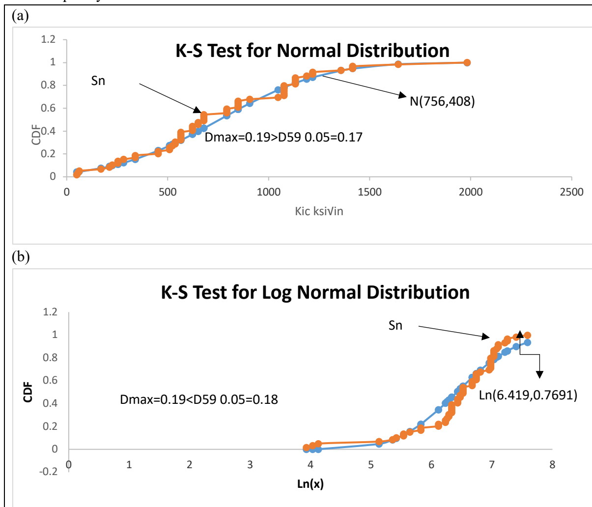
FIGURE 3: K-S TEST
