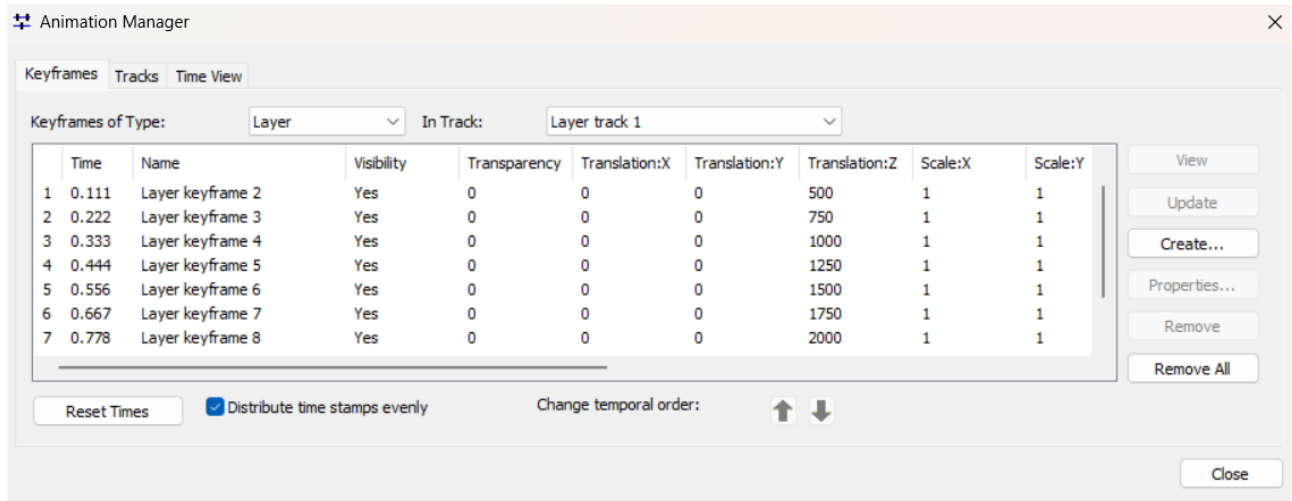
FIGURE 10: ANIMATION MANAGER
