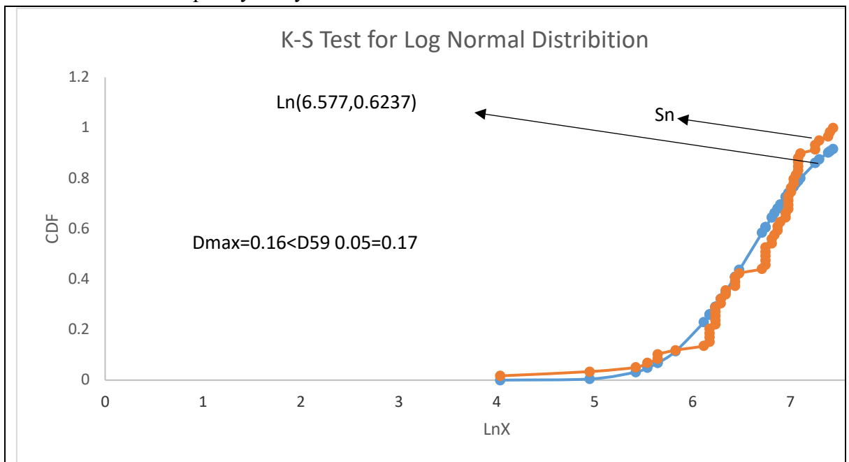
FIGURE 8: K-S TEST FOR LOG NORMAL DISTRIBUTION
