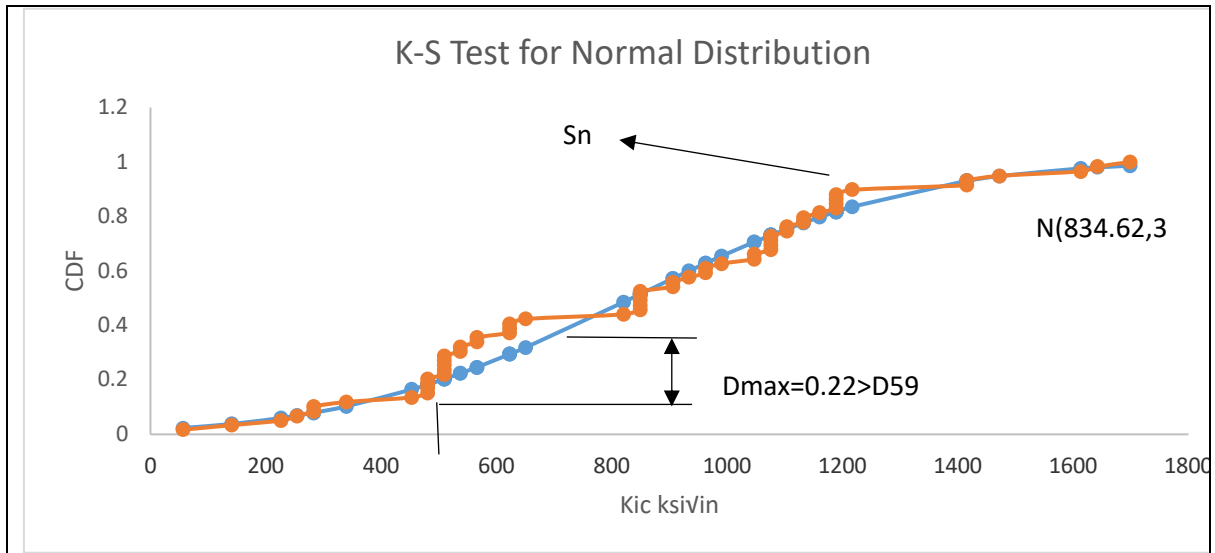
FIGURE 7: K-S TEST
