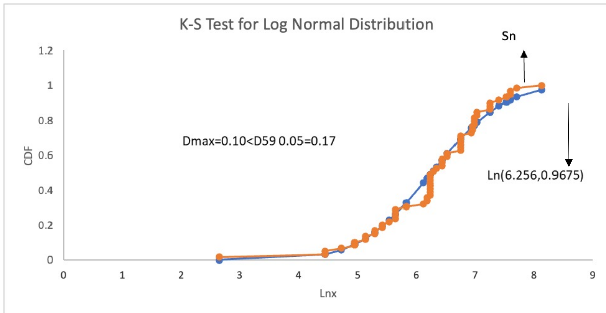
FIGURE 6: GRAPH 4 (B): K-S TEST
