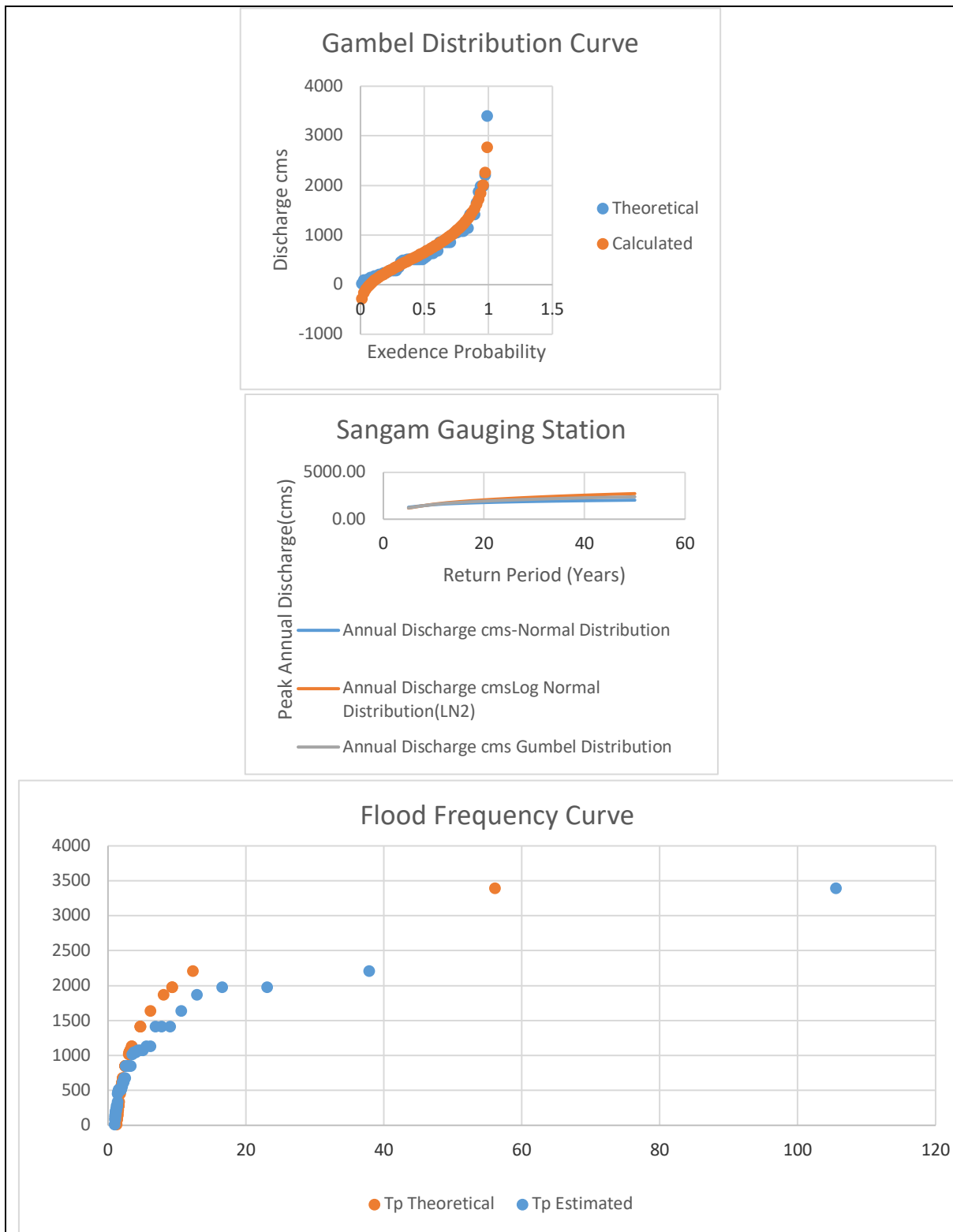
FIGURE 4: ANALYSIS OF FLOOD FREQUENCY AND DISCHARGE PREDICTIONS FOR SANGAM GAUGING STATION
